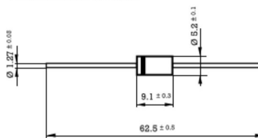
DO-201 AD (Plastic)
