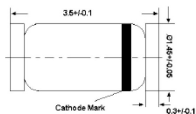
Glass Case MELF Dimensions in mm
