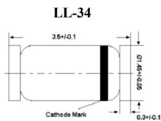
Glass Case MELF Dimensions in mm
