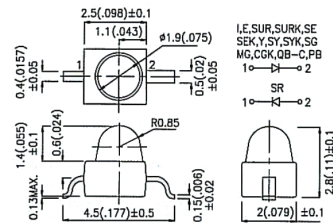
Subminiature Solid State Lamps Gull Wing Lead
