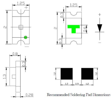
Package Outline Dimensions:
