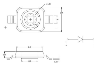
Package Dimensions
