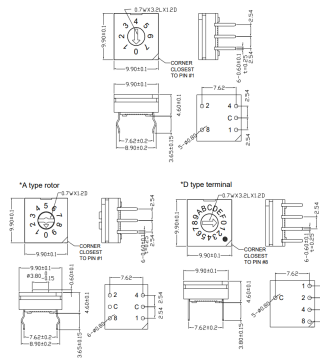
R9 - H/D (Thru-Hole)
