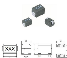
EXTERNAL DIMENSIONS (Unit:mm)
