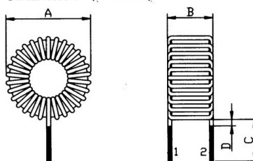
DIMENSIONS (UNIT: mm)
