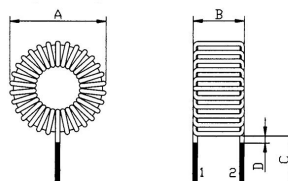
DIMENSIONS (UNIT: mm)
