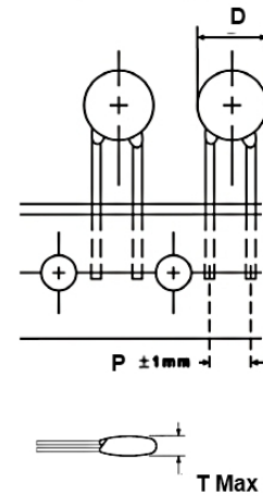
Sright Lead type
