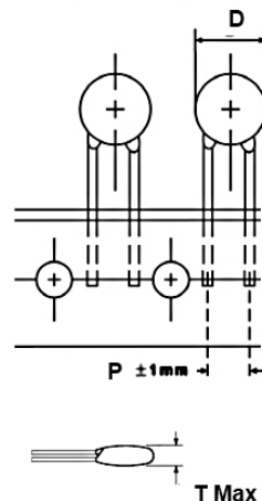
Stright Lead type
