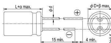
Lead Spacing and Diameter
