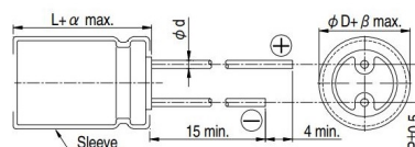
Lead Spacing and Diameter Unit: mm
